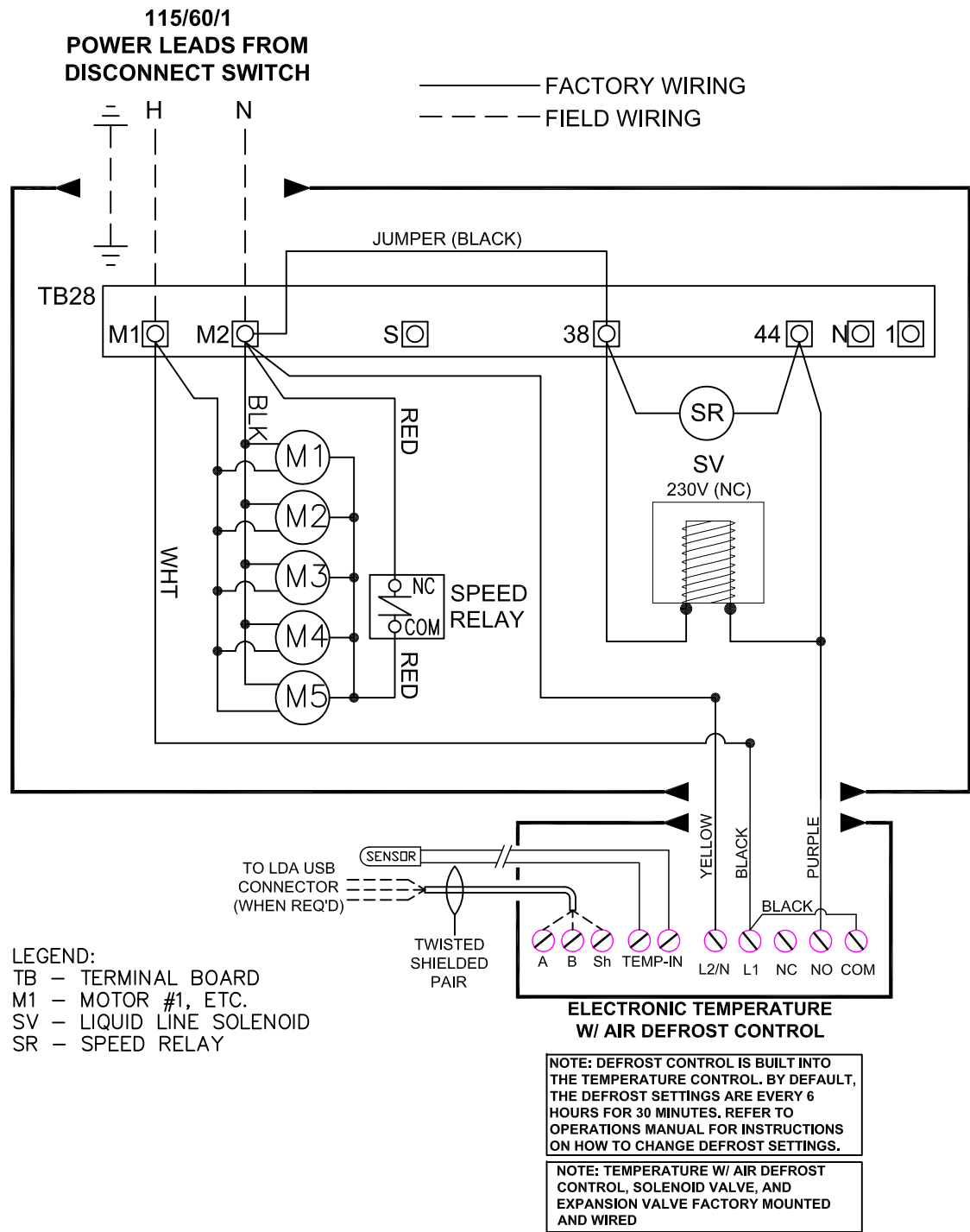
CENTER MOUNT AIR DEFROST WIRING DIAGRAM A.F.TEMP CONTROL - (115/1/60)
