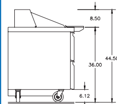
D4460NP-24M Right Side View
