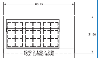
D4460NP-18M Pan Cutout Configuration
