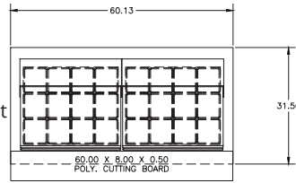
4460NP-24M Pan Cutout Configuration
