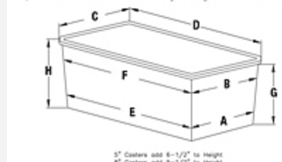
PlasticBox-Dimensions
