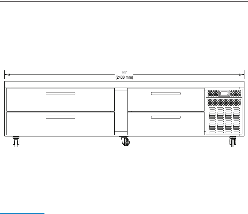
FRONT VIEW
