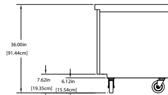
TYPICAL END
