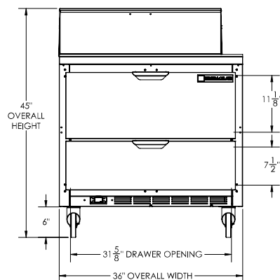
ELEVATION VIEW
