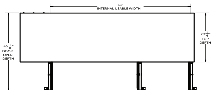
ELEVATION VIEW
