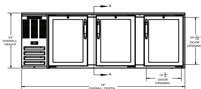
ELEVATION VIEW
