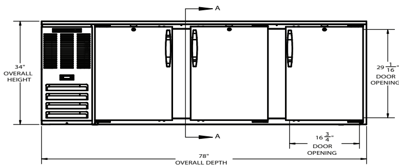
ELEVATION VIEW
