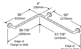
TWO-WALL WHEELCHAIR TOILET COMPARTMENT
