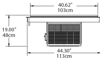
Elevation View
