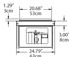
Right End View
