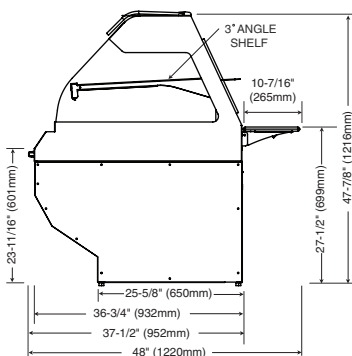
ED2SYS-72/2S Profile
