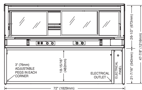
ED2SYS-72/2S Back View
