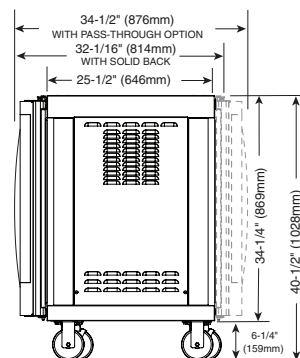
SIDE VIEW - DOUBLE PANE, CURVED DOOR, SOLID BACK
