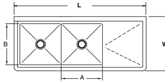
2 COMP - 1 DRBD
