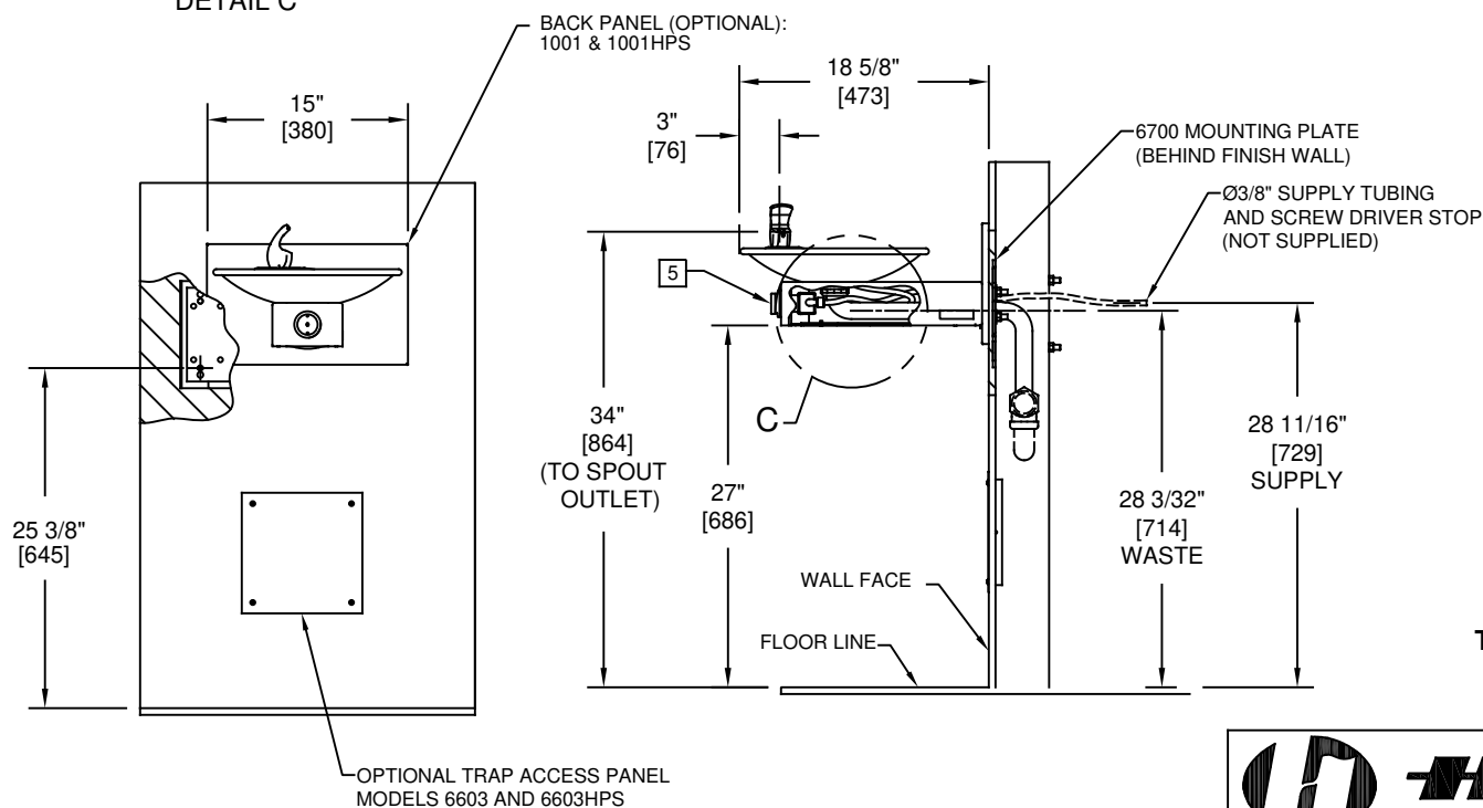
DETAIL C
