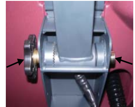
Align the teeth on the bushing and handle assembly before tightening the adjustment knob.
