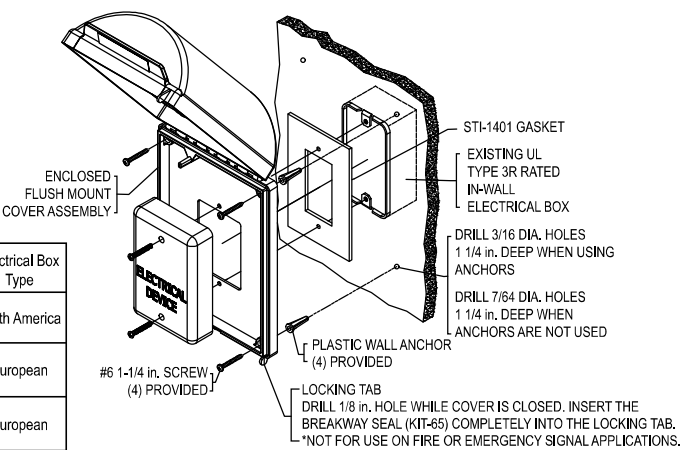
Fig. 5 - Enclosed Flush Mounting Option - Models 133** & 143** NEMA TYPE 3RX
