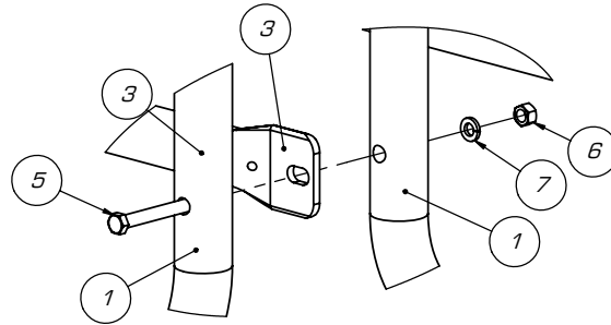
DETAIL B SCALE 1 : 6
