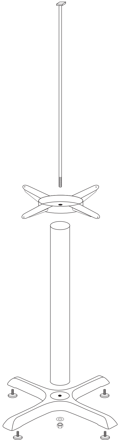
ASSEMBLY DIAGRAM
