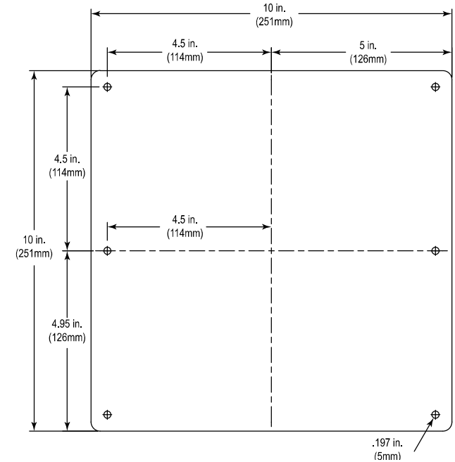
BACKPLATE STI-MBP1010
