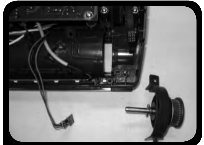
10. Remove clutch assembly
