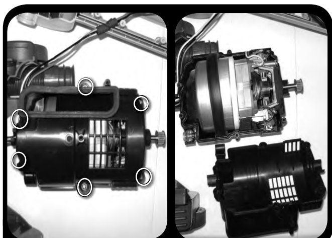
11. Remove upper motor housing - Remove six (6) (M4 x 16mm length) screws
