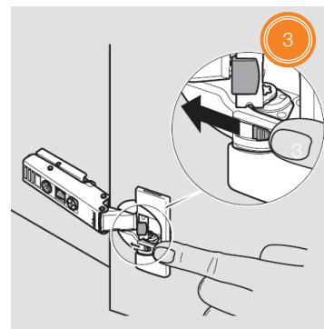
CLIP TOP BLUMOTION DEACTIVATION
