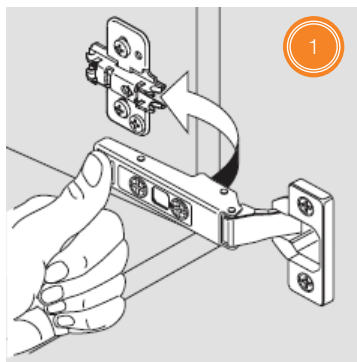
DOOR INSTALLATION
