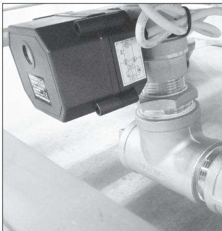
Fig. 6B - Electric Drain Valve
