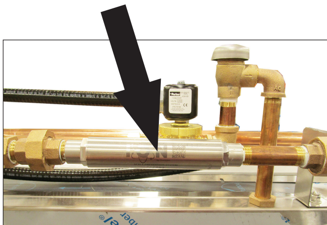
Fig. 7b - Ion Water Conditioner Installed
