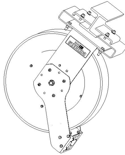
MRT-1: T &amp; C SERIES MOUNT KIT
