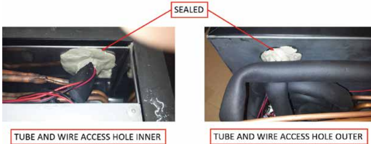
Figure 6-15.9. Seal Access Hole
