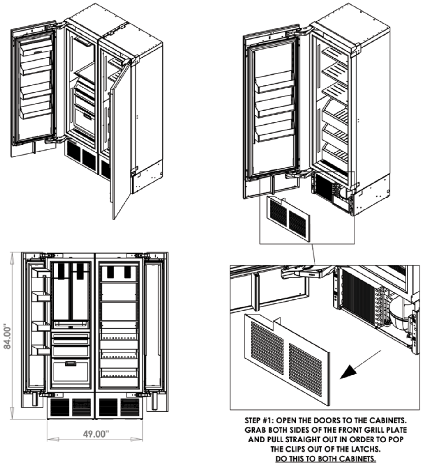
Figure 8-23.1. Marriage Kit Install (1)
