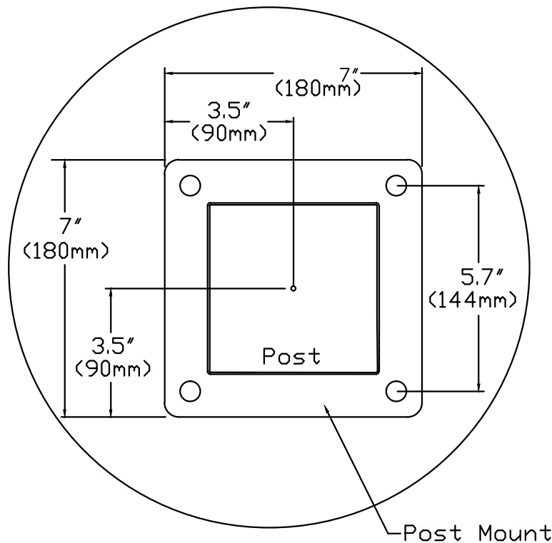
Post Detail
