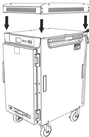
Lower Cabinet
