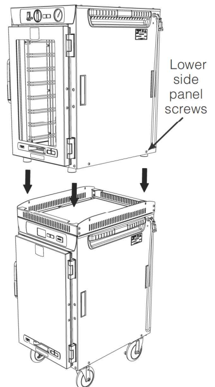
Stacking Cabinets
