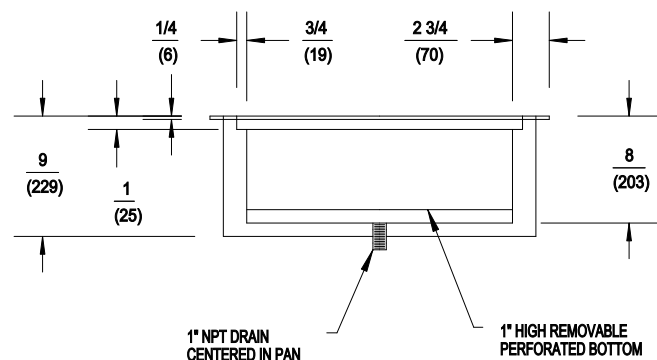
CROSS-SECTION OF COLD PAN
