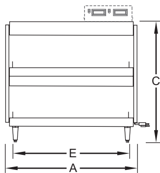
GRSDH—Dual Shelf
