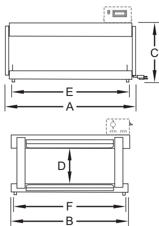
GRSDH—Single Shelf
