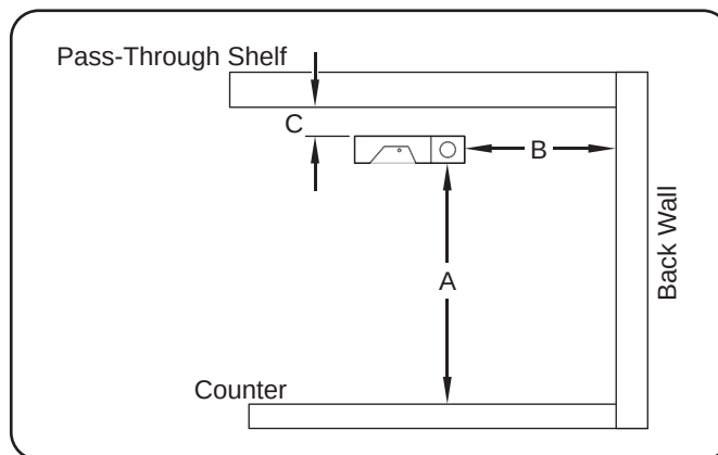
Combustible Clearance Requirements
