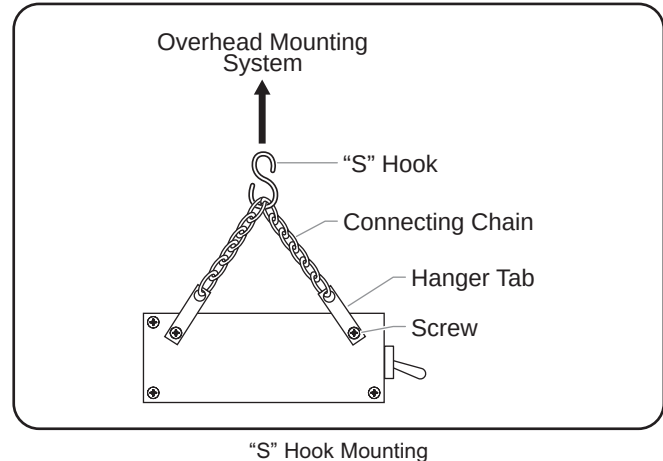
"S" Hook Mounting
