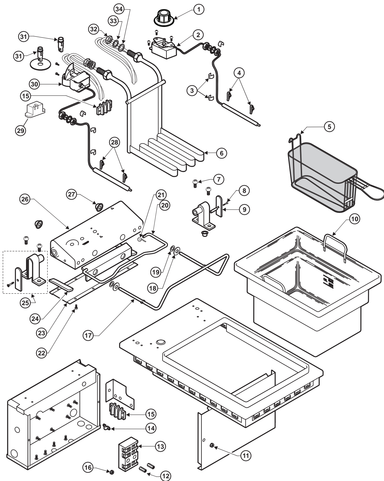
Model: F-556 Single Head Built-In Standard Fryer
