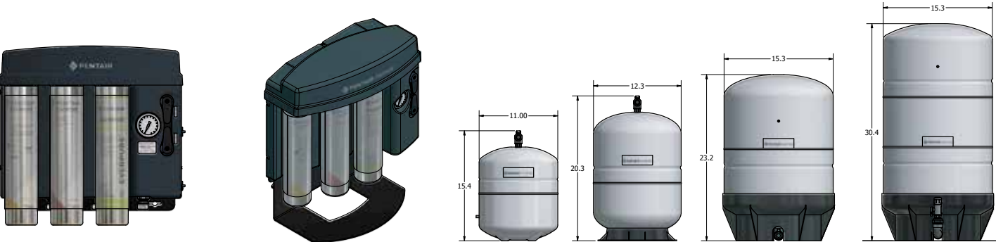
Wall-mounted EZ-RO processor EZ-RO on (optional) floor stand Hydropneumatic tank sizes, depending on model purchased: 2 gal, 5 gal, 10 gal, 16 gal
