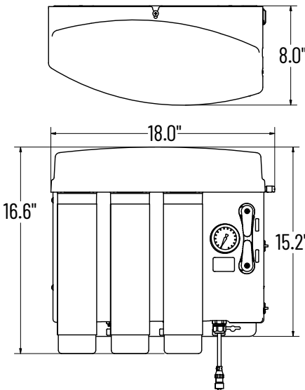
Processor with Size 4 Cannisters, Wall Mounted
