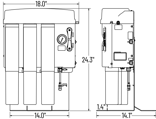
Processor with Size 7 Cannisters on Optional Stand
