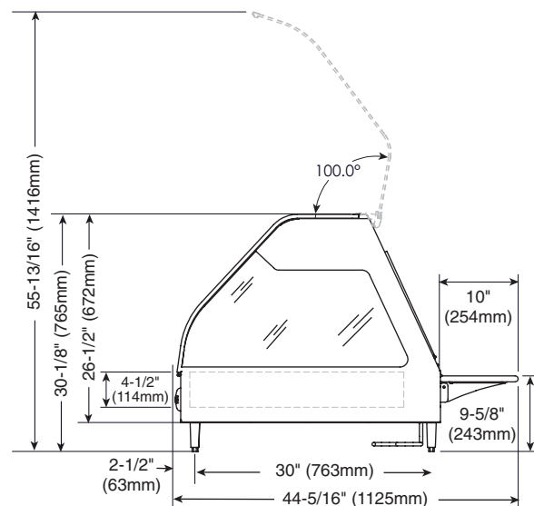
ED2 PROFILE
