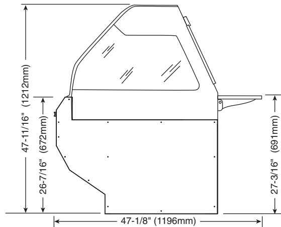
ED2SYS PROFILE
