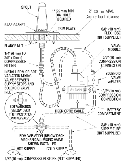
EBF-85 Faucet with BDM/BDT Variation Mixing Valves
