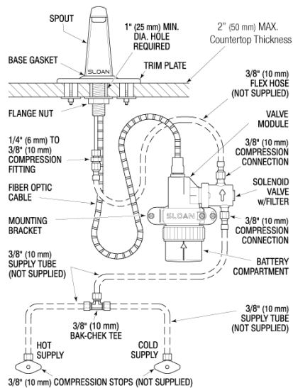
EBF-85 Faucet with Bak-Chek Tee
