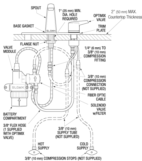
EBF-85 Faucet with ADM Variation Mixing Valve
