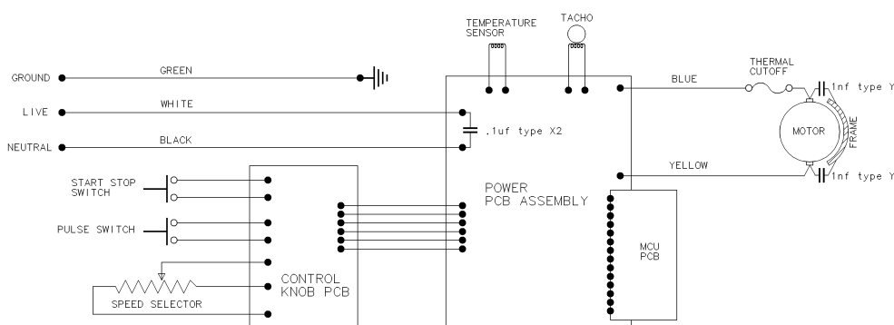
Wiring Diagram
