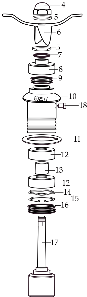
502977 Blending Assembly (replaces 502493 or 502975)
