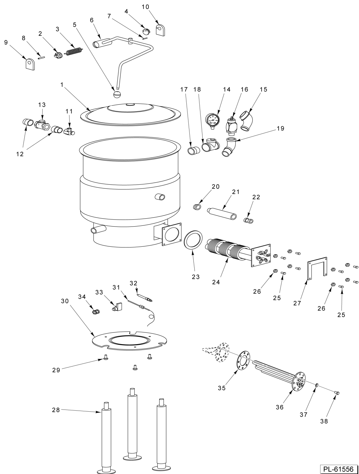
K20EL, K40EL AND K60EL COMPLETE ASSEMBLY
