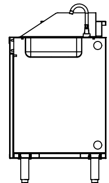
SECTION H-H
