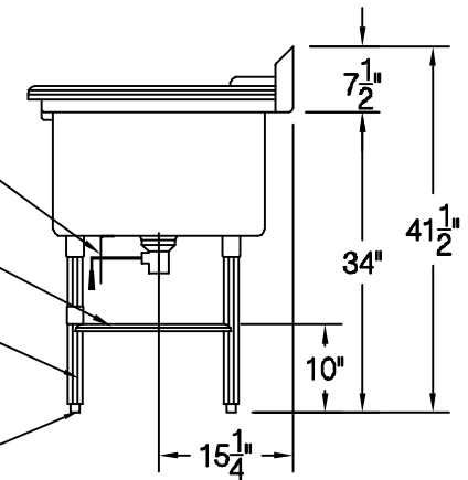
Splash Detail
