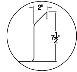
Splash Detail
