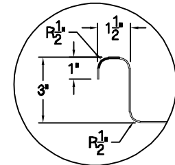
Roll Detail
