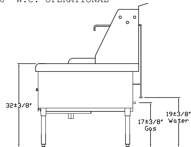
GENERIC SIDE VIEW
