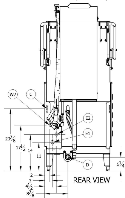
SINGLE POINT ELECTRICAL CONNECTION
