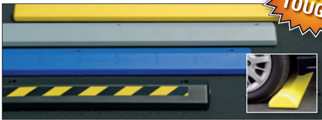
Model 1790Y Parking Stop - Yellow / 8" w x 4" h x 72" l
