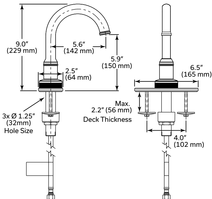
With Black Spacer
