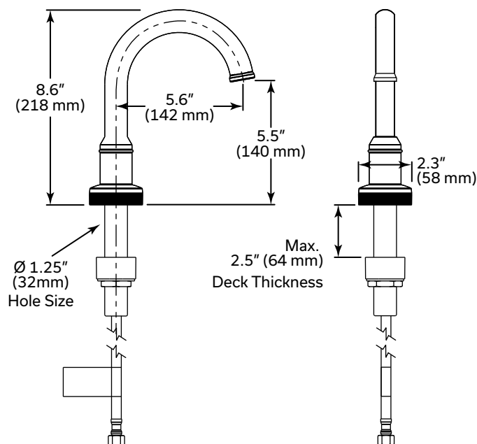
Single Hole with Black Spacer
