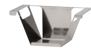
burner holder 12.2171.0000 ♥ 10.2" x 7.8" x 3.8" for all stands GN 1/1 and induction plus
