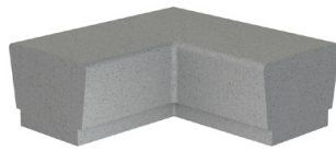
5. WS909 CORNER, 90° SQUARE 48" x 48" x 18" 2,550 lbs.
