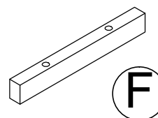
RAIL Riel RAIL T9320196061JH QTY: 2
