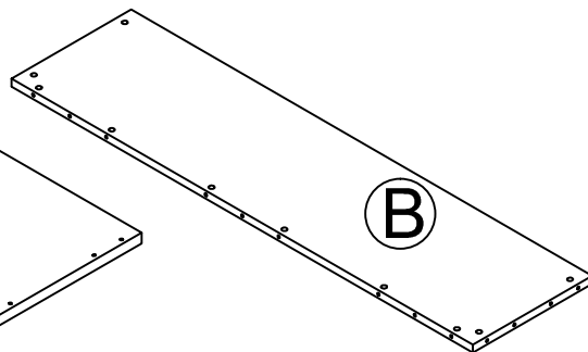
BACK PANEL Panel trasero PANNEAU ARRIÈRE T9319196022JH
