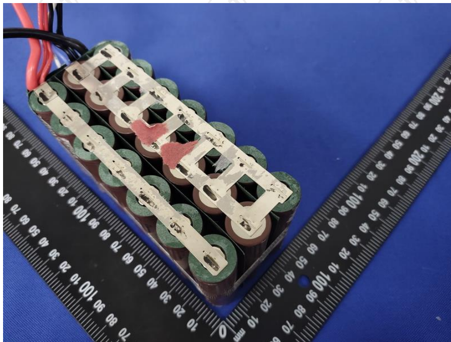
Picture 5. Battery view
