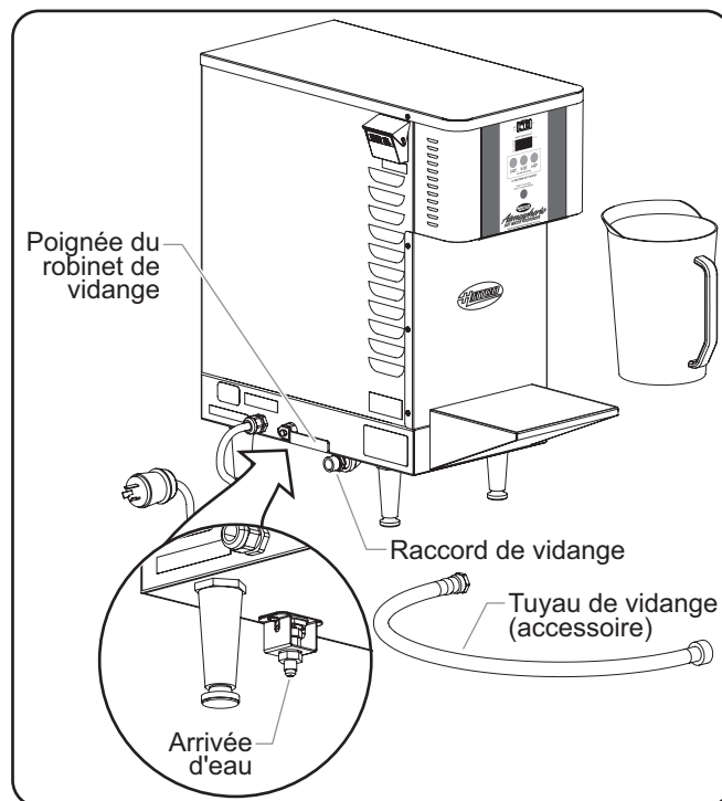
Installation AWD-12
