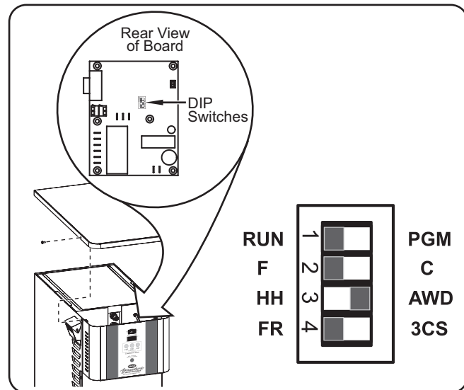
Dipswitch Controls
