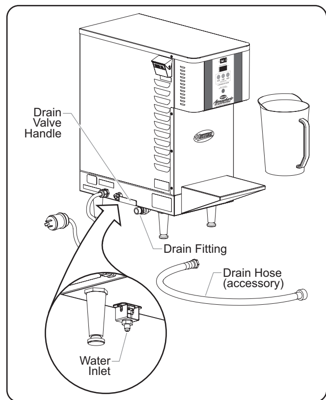
AWD-12 Installation
