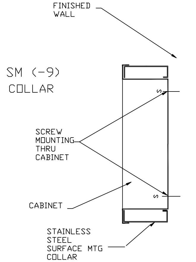
CABINET AND COLLAR ASSEMBLY ARE THEN MOUNTED TO WALL
